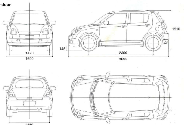
Dimensions (mm)
